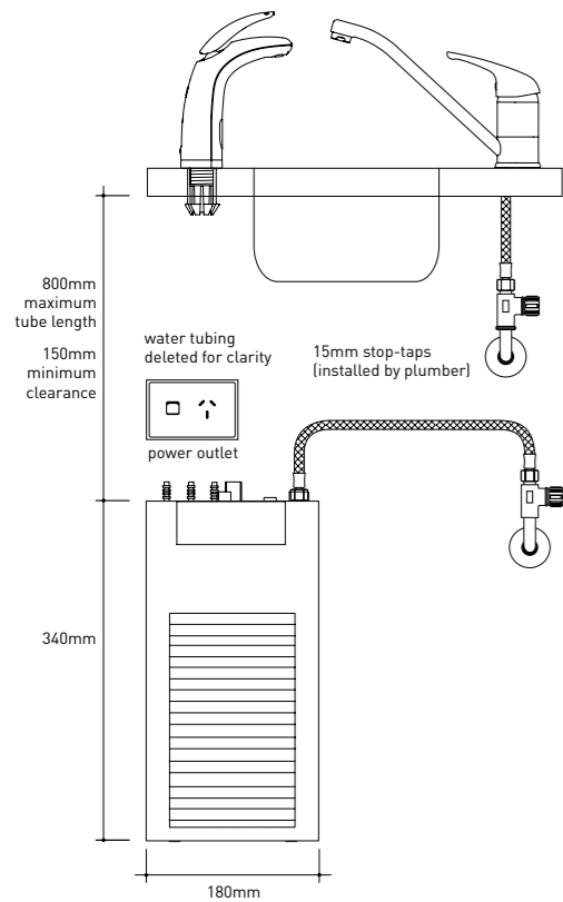
Preferred installation layout
